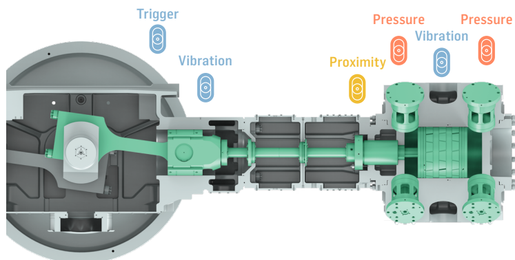
Modular monitoring system: selection of vibration, pressure and proximity sensors
