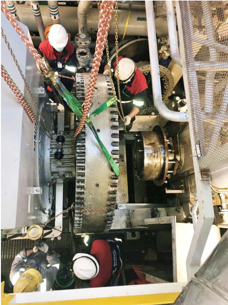
Burckhardt Compression experts working on the compressor skid in the confines of the compressor machinery room (CMR).
